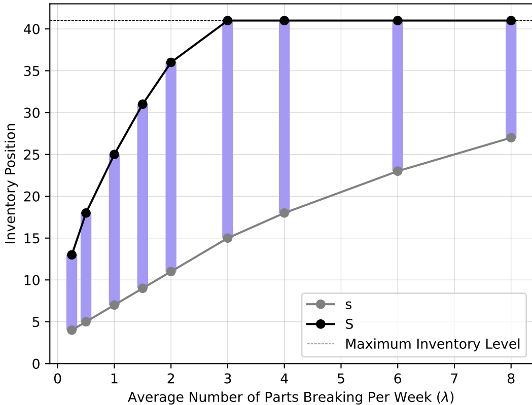
Optimal (s, S) Policies for Different Demand Intensities ( p=0.9 )
