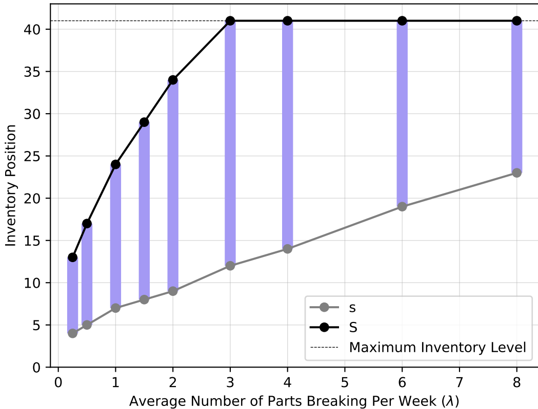
Optimal (s, S) Policies for Different Demand Intensities ( p=1.0 )
