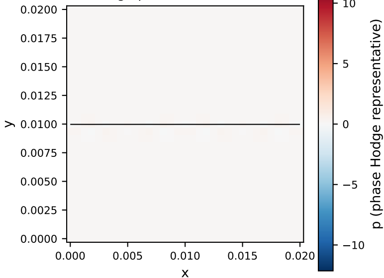
Hodge pressure at t = 0.009
