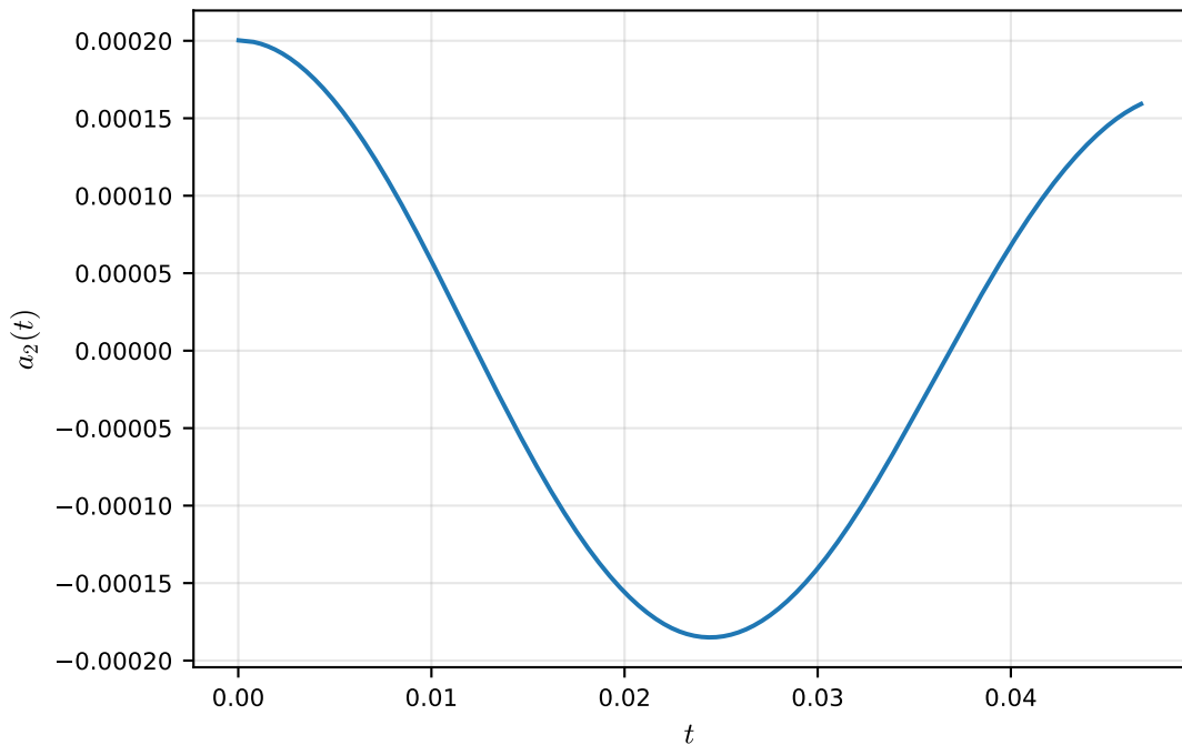
Water-air capillary wave: signed mode amplitude
