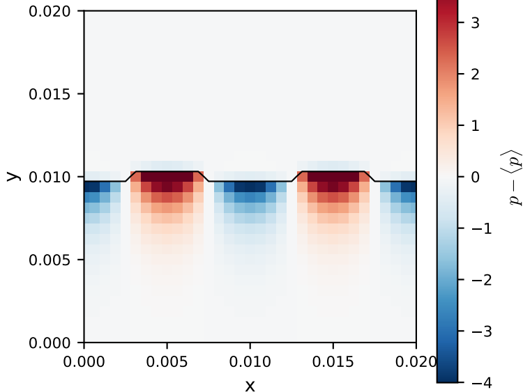
Pressure at t = 0.023
