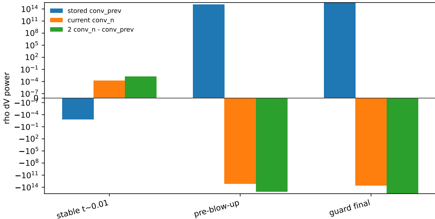
UCCD6 IMEX-BDF2 history power
