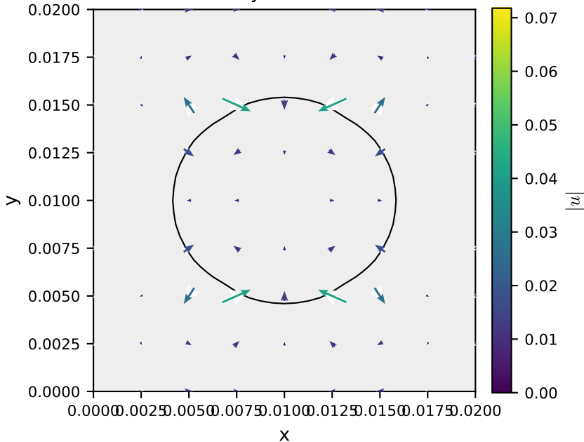
Velocity at t = 0.105
