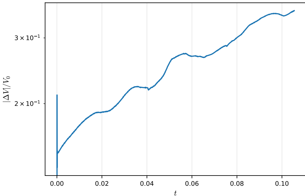
Rayleigh-Lamb n=2 droplet: volume drift
