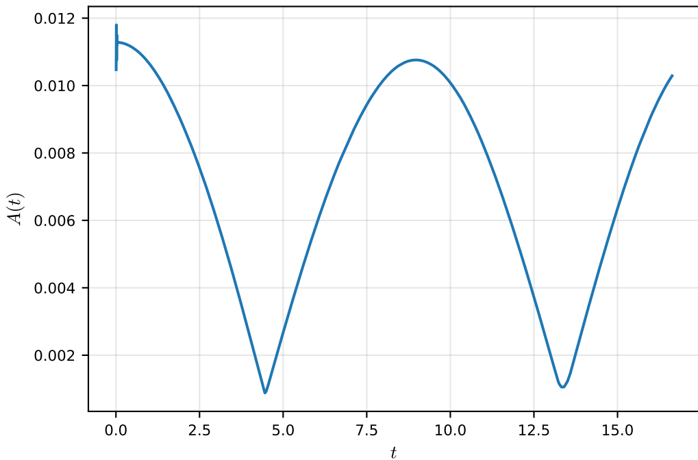
Water-air capillary wave: interface amplitude
