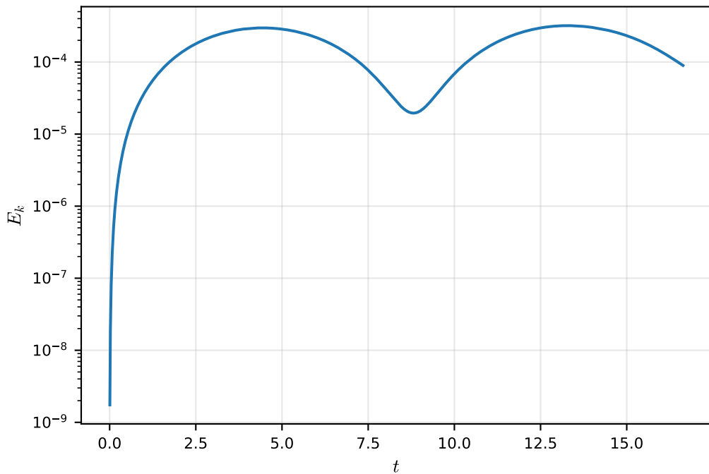
Water-air capillary flow: kinetic energy
