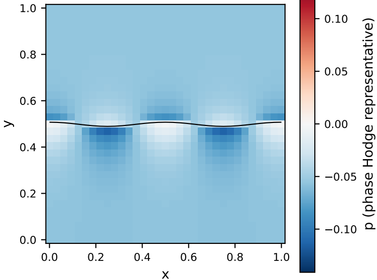
Hodge pressure at t = 16.633
