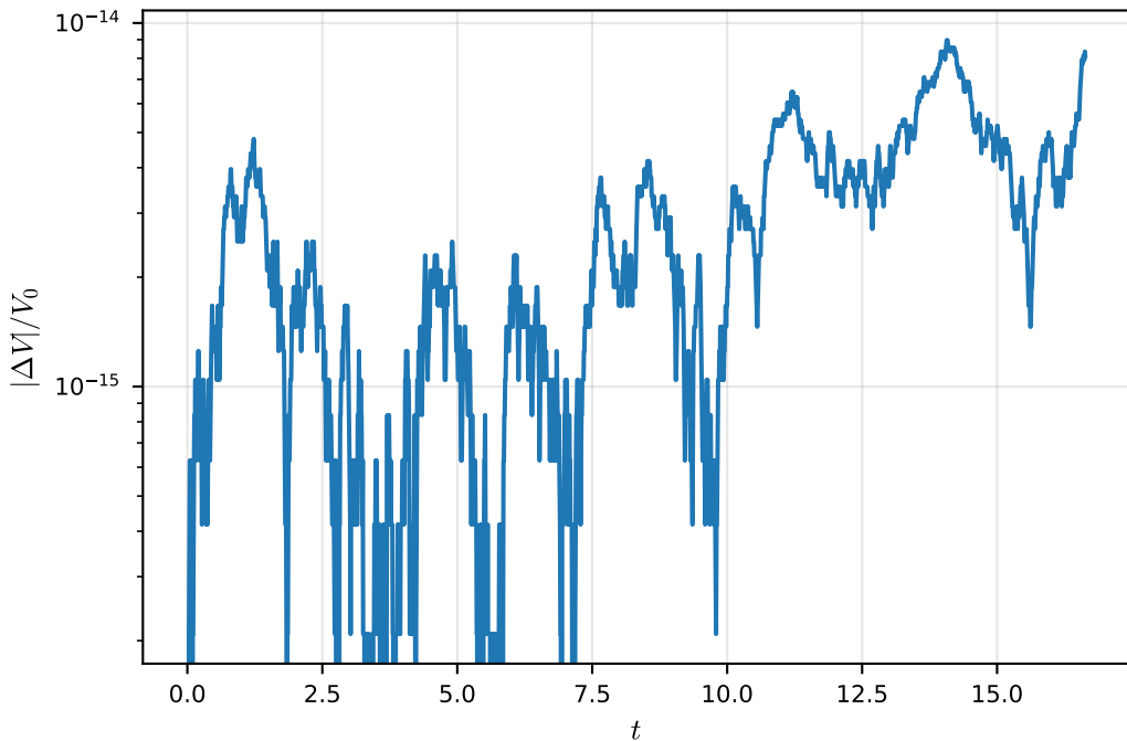
Water-air capillary flow: volume drift
