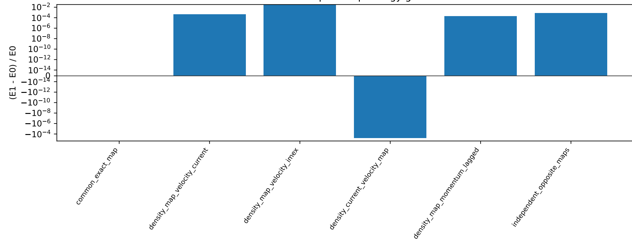
Exact transport map energy gate
