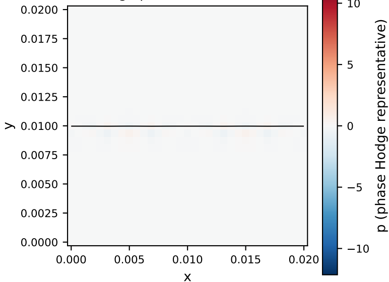
Hodge pressure at t = 0.027
