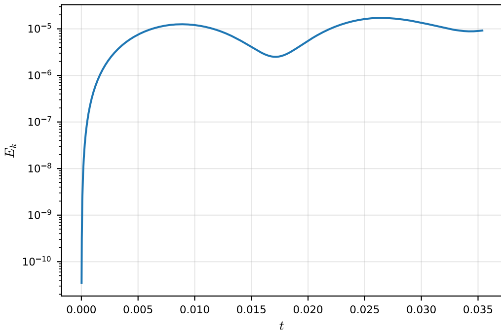
Water-air capillary flow: kinetic energy
