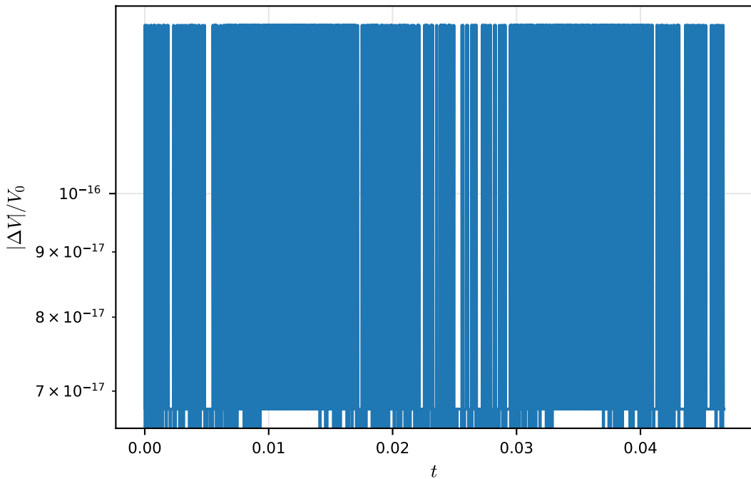
Water-air capillary flow: volume drift
