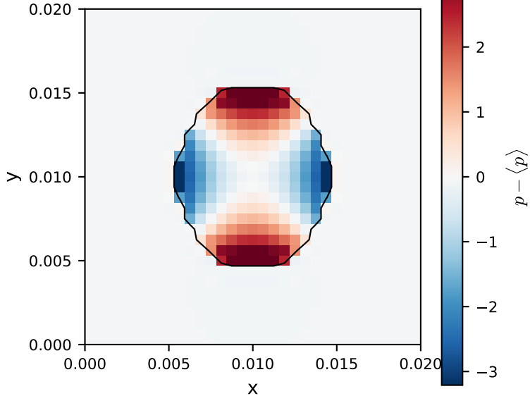
Pressure at t = 0.053
