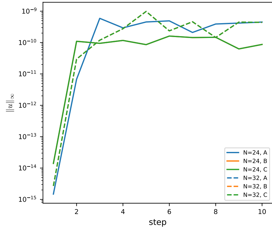
V9 §14 stack: spurious-current trajectory
