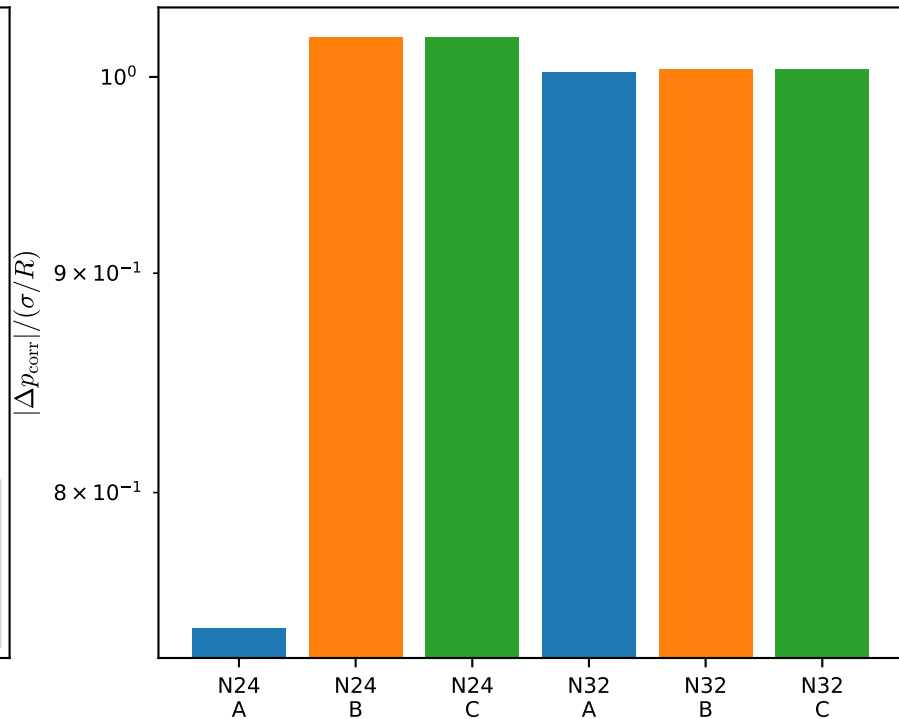
V9 §14 stack: pressure-corrector contrast
