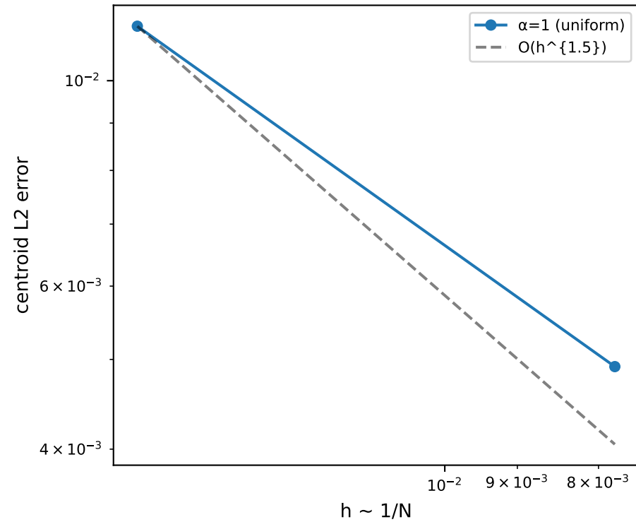
V10: Zalesak rotation centroid
