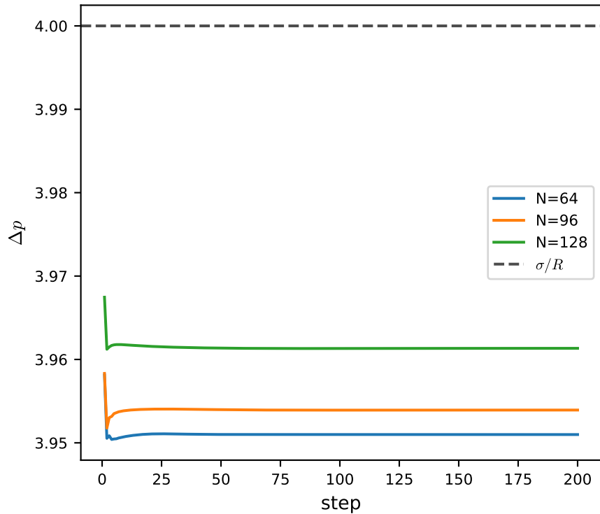
Laplace pressure (200 step)
