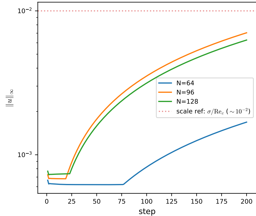
Spurious current trajectory (200 step)
