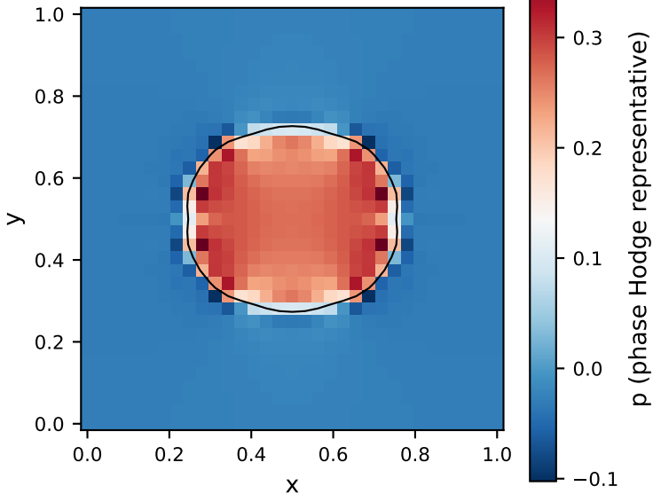
Hodge pressure at t = 37.526
