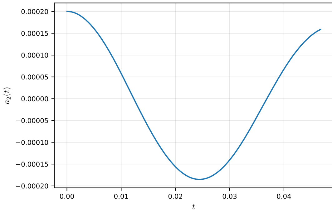
Water-air capillary wave: signed mode amplitude
