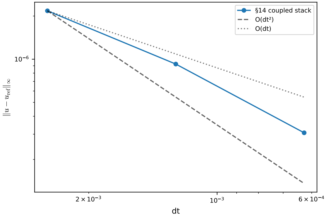
V7: §14 stack time-order diagnostic (N=24)
