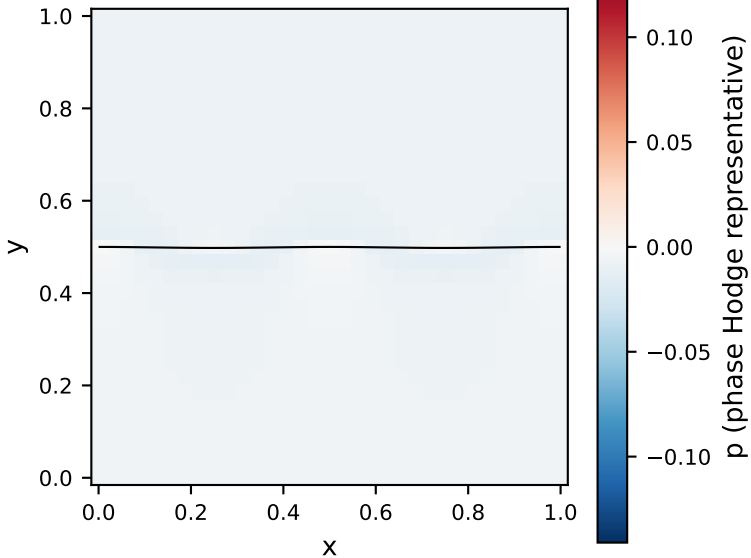
Hodge pressure at t = 4.160
