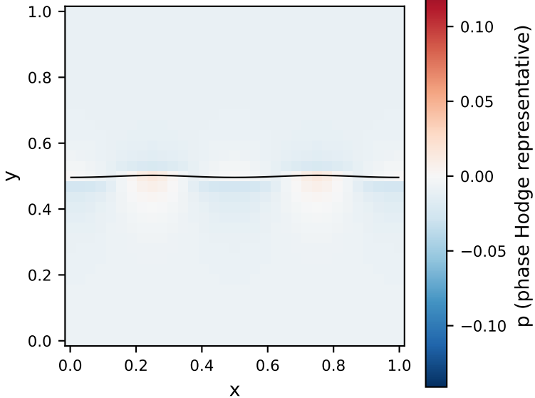
Hodge pressure at t = 12.480
