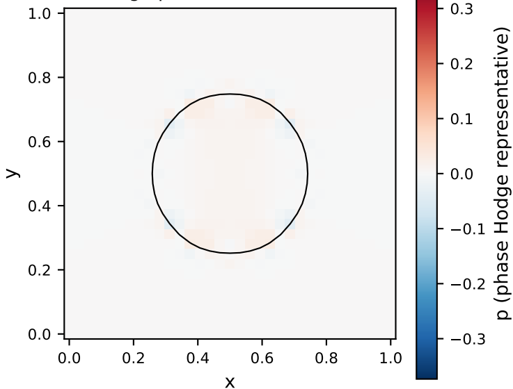
Hodge pressure at t = 28.152
