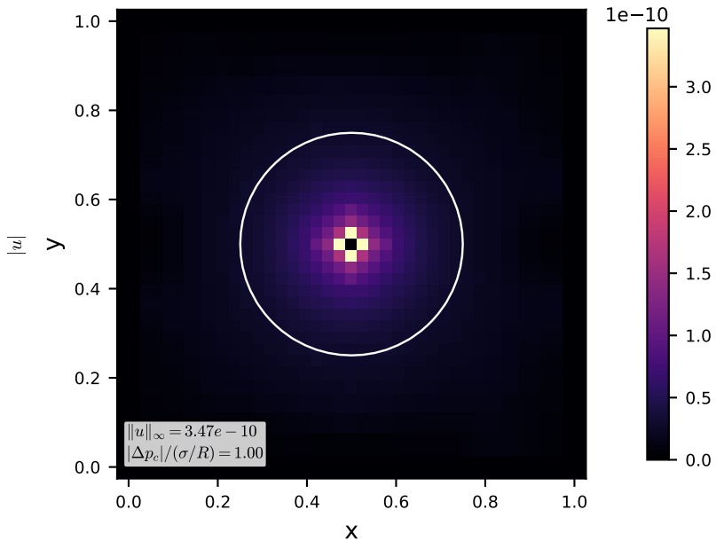
B: \alpha=2 , nominal \epsilon
