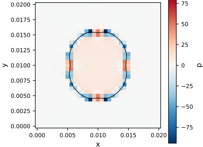
Pressure at t = 0.053
