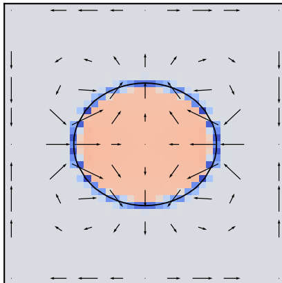
p-mean + velocity, |u|_{\max}=8.97e-03
