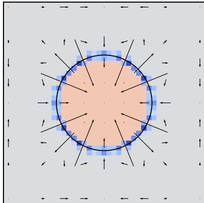
Oscillating droplet psi t=2.50
