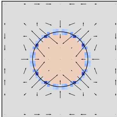
Oscillating droplet psi t=5.01
