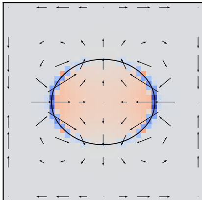
p-mean + velocity, |u|_{\max}=6.97e-03
