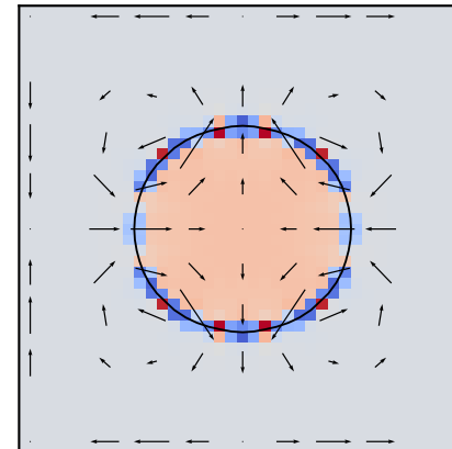
p-mean + velocity, |u|_{\max}=5.93e-03
