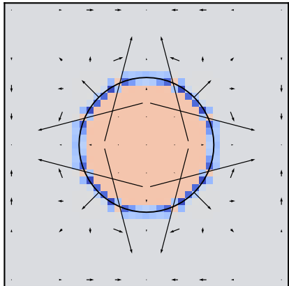
Oscillating droplet psi t=0.01
