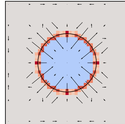
Oscillating droplet psi t=10.00
