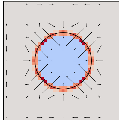
Oscillating droplet psi t=7.50
