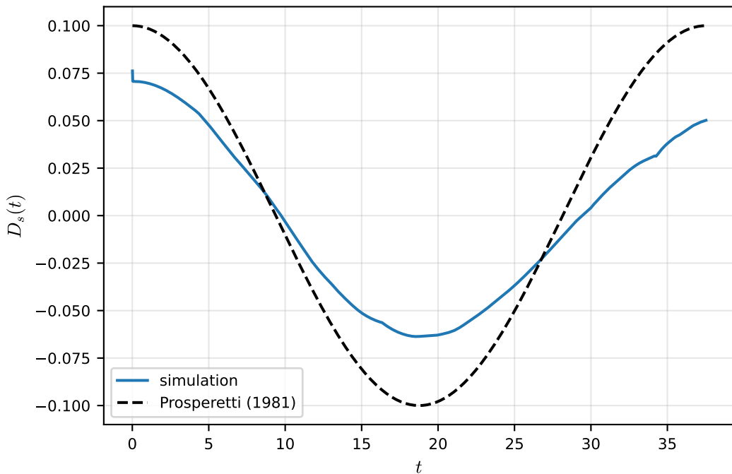
Rayleigh-Lamb n=2 droplet: signed deformation
