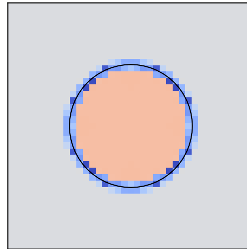
Oscillating droplet t=1.000
