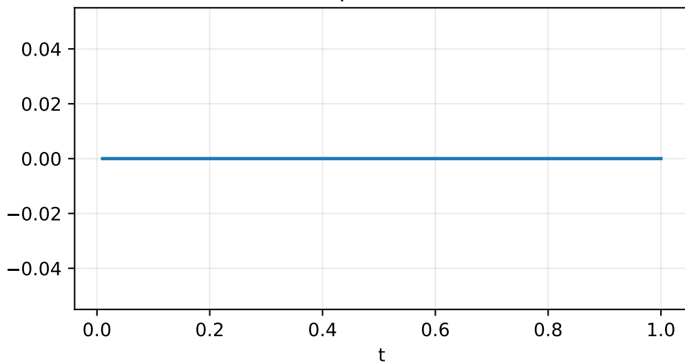
Static droplet: kinetic energy
