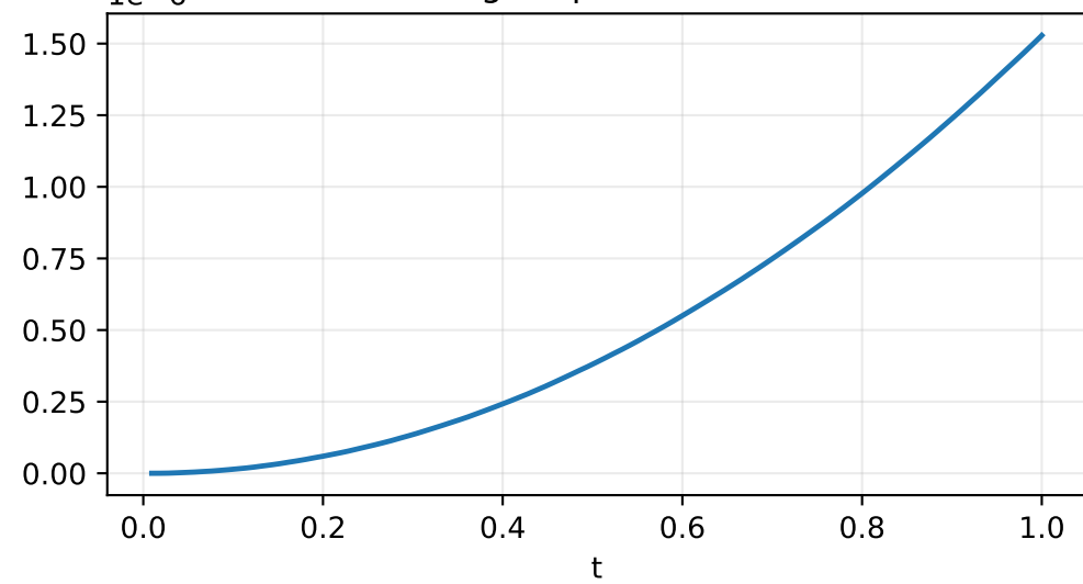
Oscillating droplet: volume drift
