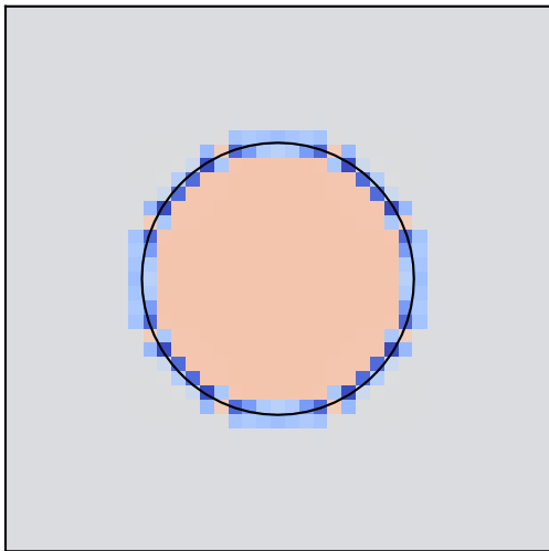
Oscillating droplet t=0.009
