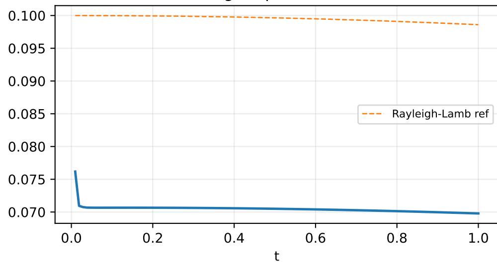
Oscillating droplet: kinetic energy
