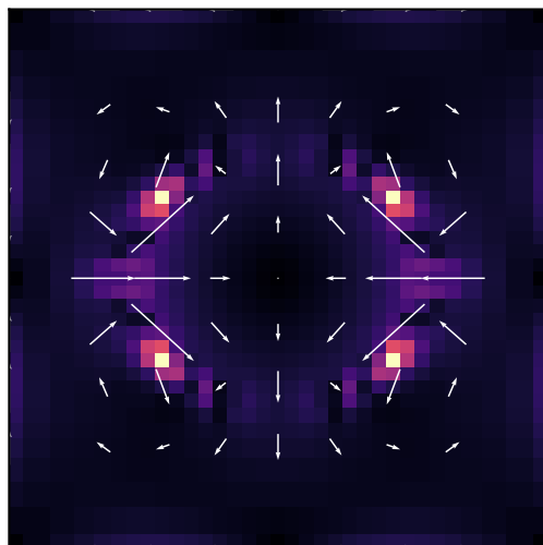
Oscillating droplet t=0.352, |u|_{\max}=1.39\text{e-}03
