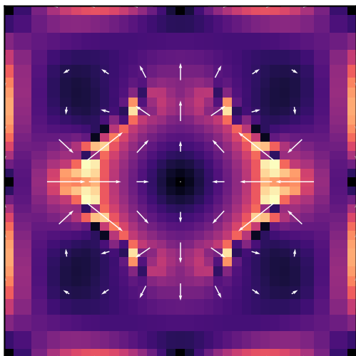
Oscillating droplet t=0.009, |u|_{\max}=1.05\text{e-}05
