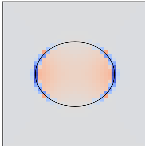
Oscillating droplet t=0.656
