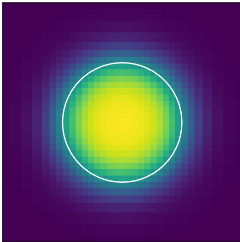
Oscillating droplet t=0.352
