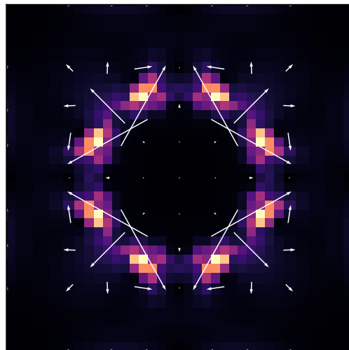
Oscillating droplet t=0.656, |u|_{\max}=2.55\text{e-}03
