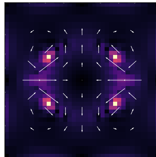
Oscillating droplet t=1.000, |u|_{\max}=3.64\text{e-}03
