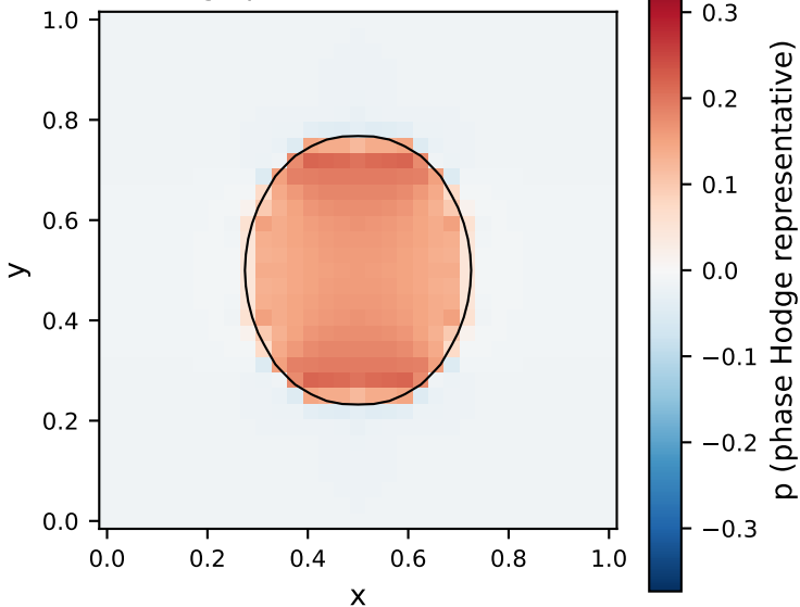
Hodge pressure at t = 18.769
