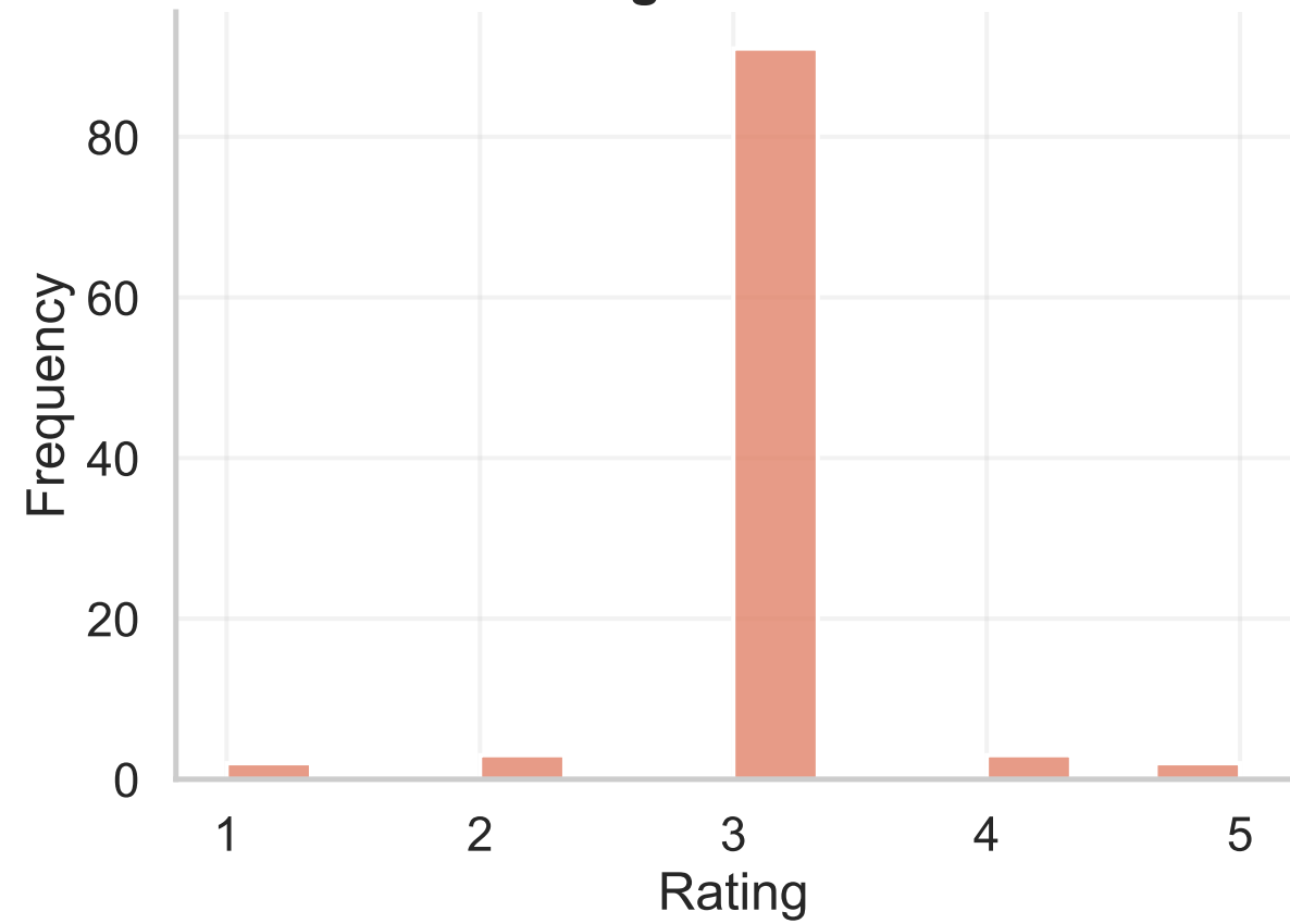
Rating Distribution
