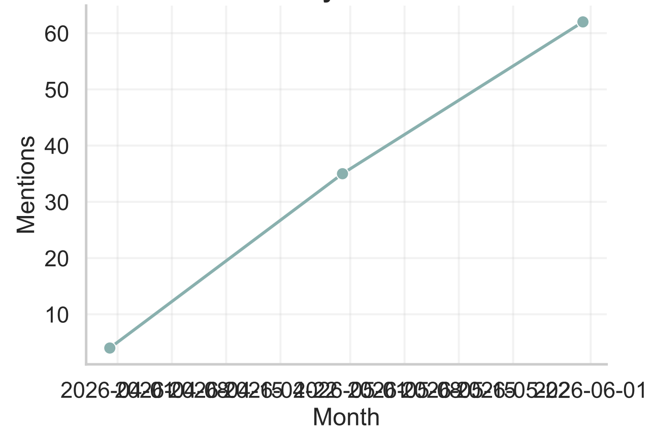
Monthly Mentions
