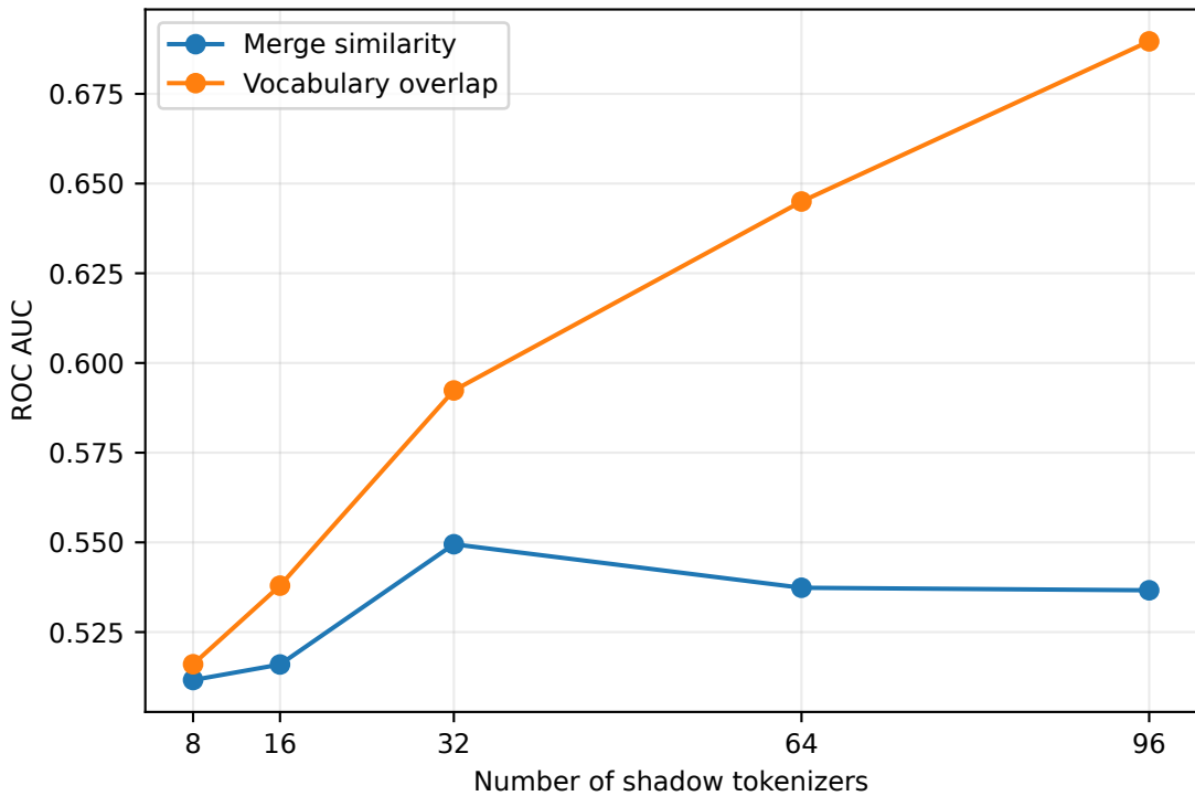
Shadow-tokenizer sensitivity
