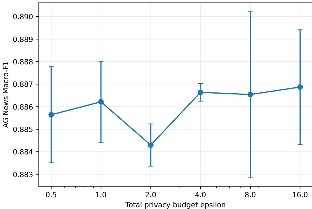
Privacy budget and downstream utility
