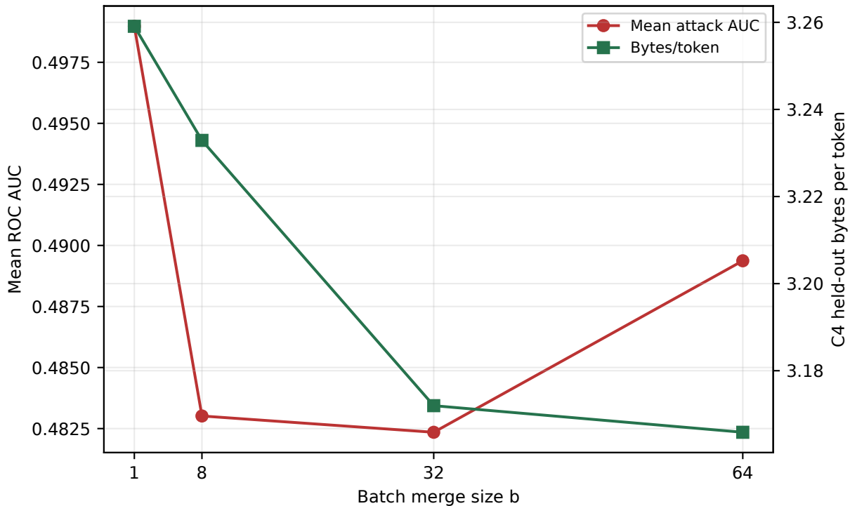
Batch-merge ablation
