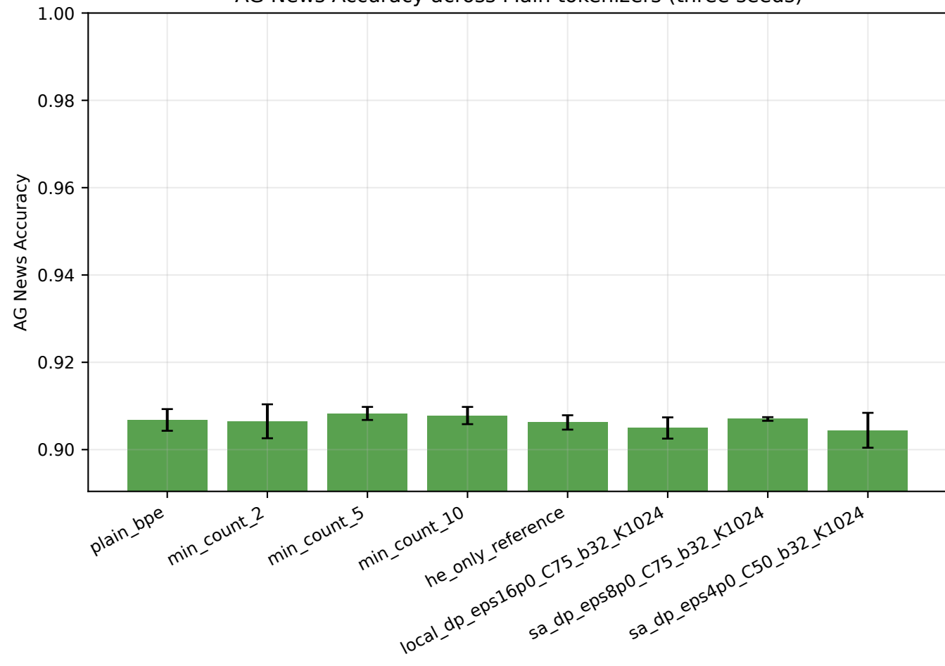
AG News Accuracy across Main tokenizers (three seeds)
