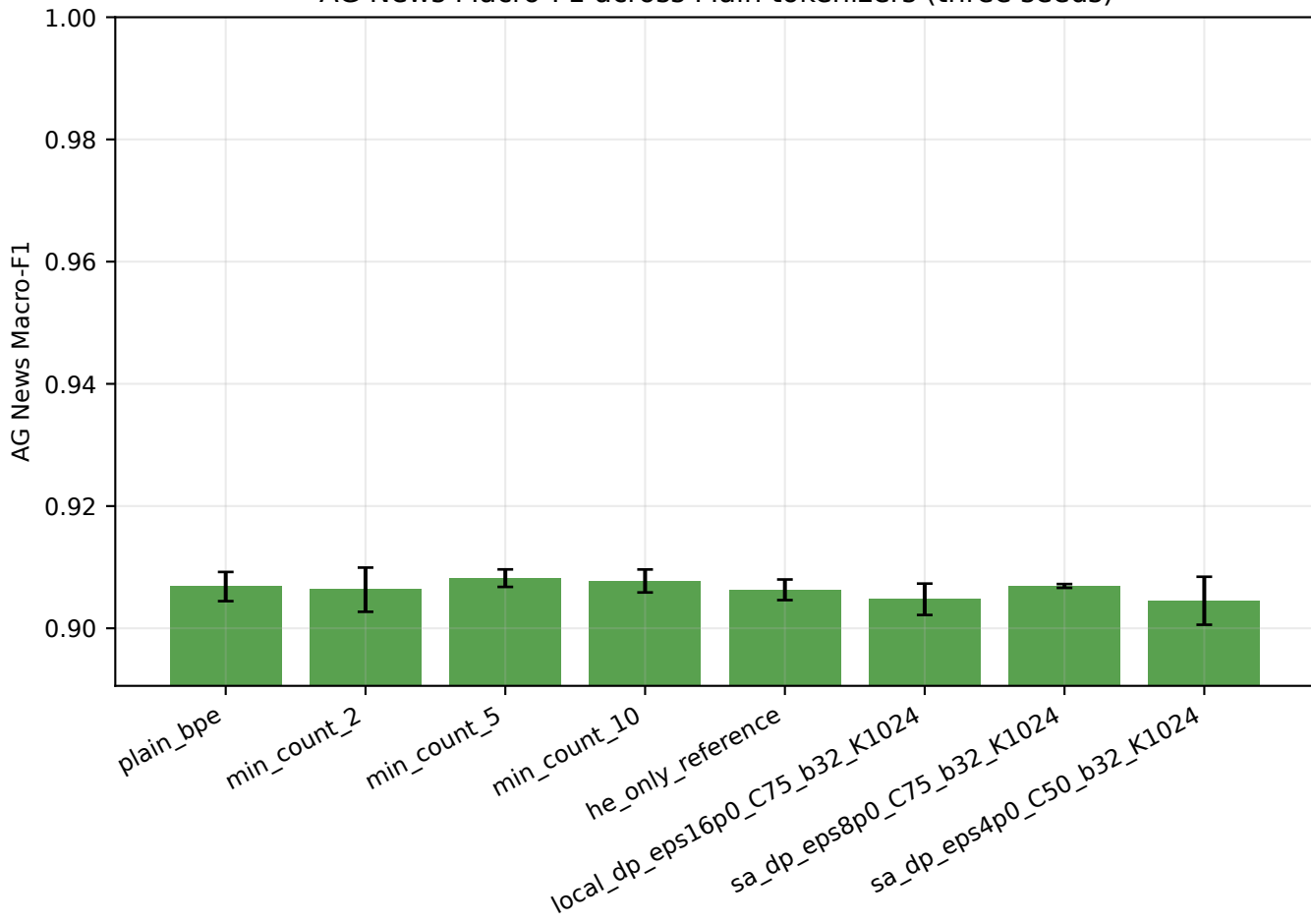
AG News Macro-F1 across Main tokenizers (three seeds)
