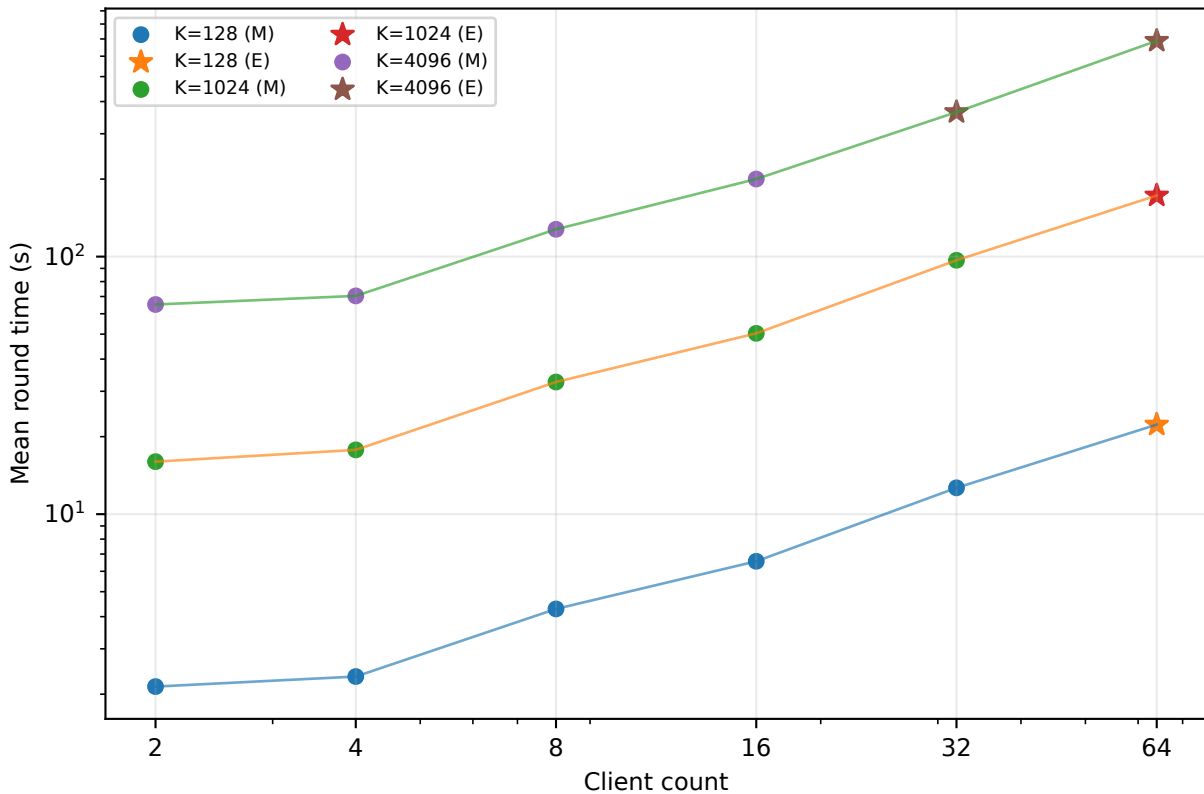
Paillier total time versus clients: measured and extrapolated
