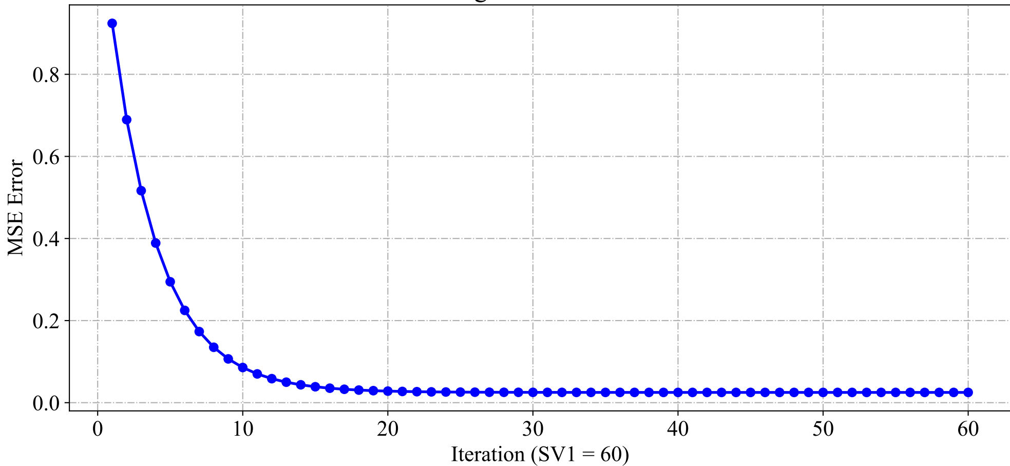
Error convergence over each iteration
