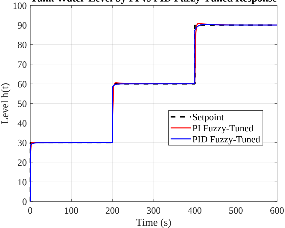
Tank Water-Level by PI vs PID Fuzzy-Tuned Response
