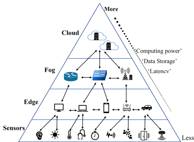
Fig. 1 A generic architecture for edge-to-cloud environments adopted from [8]
