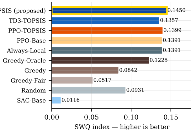
(b) SWQ = \hat{\tau} \cdot \overline{slack}
