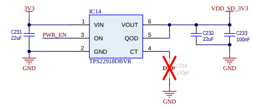
uSD Card Load Switch
