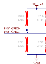
Ethernet PHY
