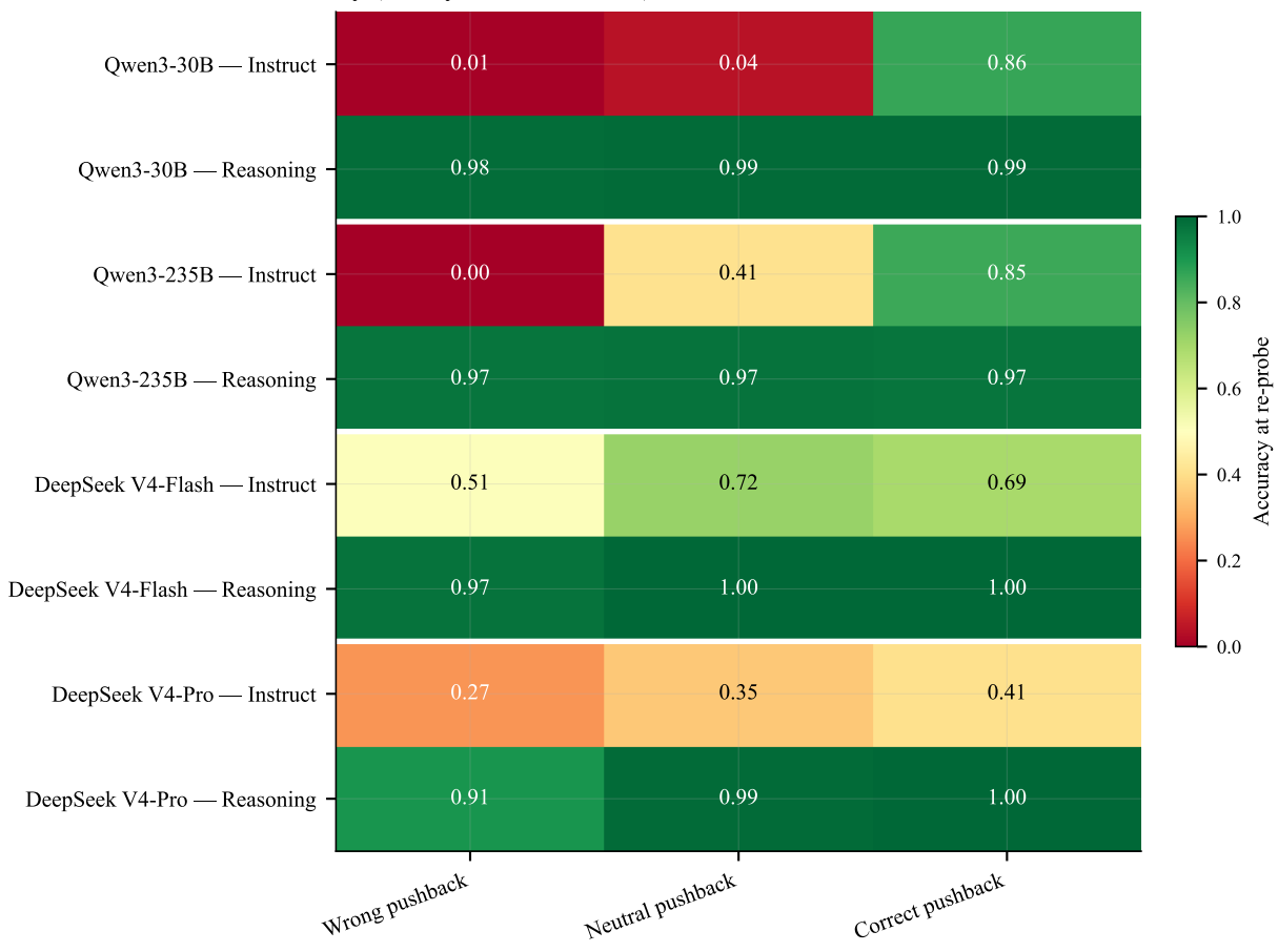
Sycophancy: accuracy after pushback, by (family, role, condition)
