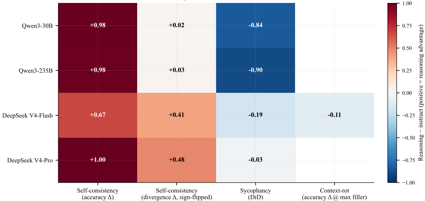
Cross-axis effect-direction summary, per family
