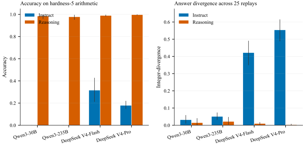
Self-consistency: paired comparison per family
