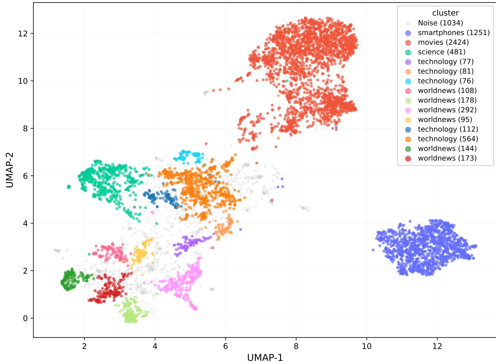
UMAP — Reddit Posts by HDBSCAN (k=14)
