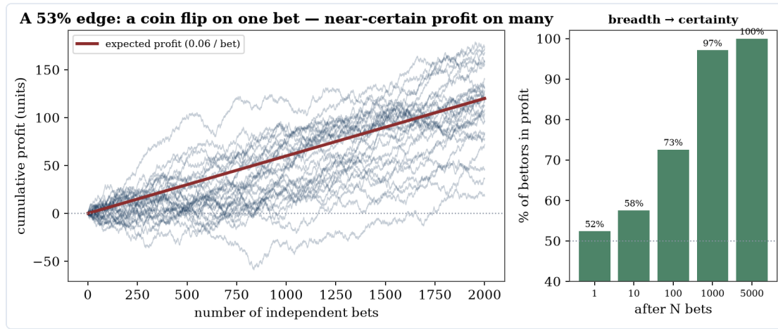
Figure 6.2. The same law as a simulation: gamblers with a tiny 53% edge scatter over a few bets but fan into reliable profit over thousands — and the share in profit climbs toward certainty with breadth. A small edge industrialised is the engine of every statistical-arbitrage fund.
