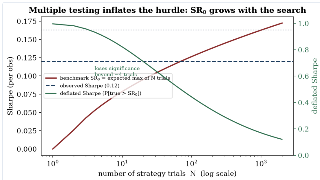
Figure 3.4. Multiple testing inflates the significance hurdle: the benchmark Sharpe grows with the number of trials, so an observed Sharpe loses significance as the search widens.
