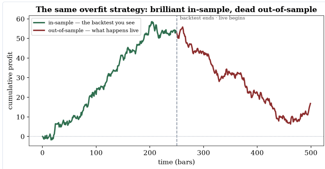
Figure 3.3. Overfitting made visceral: the same strategy soars on the data it was tuned to and collapses the moment it meets data it has never seen. The vertical line is where the backtest ends and reality begins.
