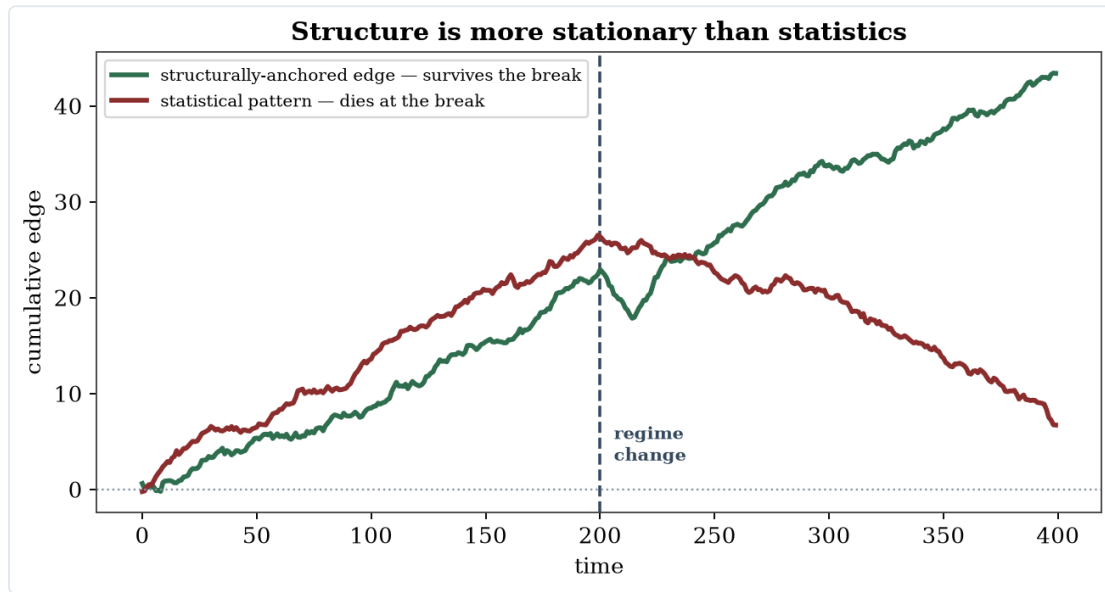
Figure 3.2. Why structure beats statistics under non-stationarity: at a regime break, a statistical pattern (a correlation that merely 'worked') dies, while an edge anchored in a durable structural counterparty takes a hit and resumes. A relationship is exactly as stationary as its source.
