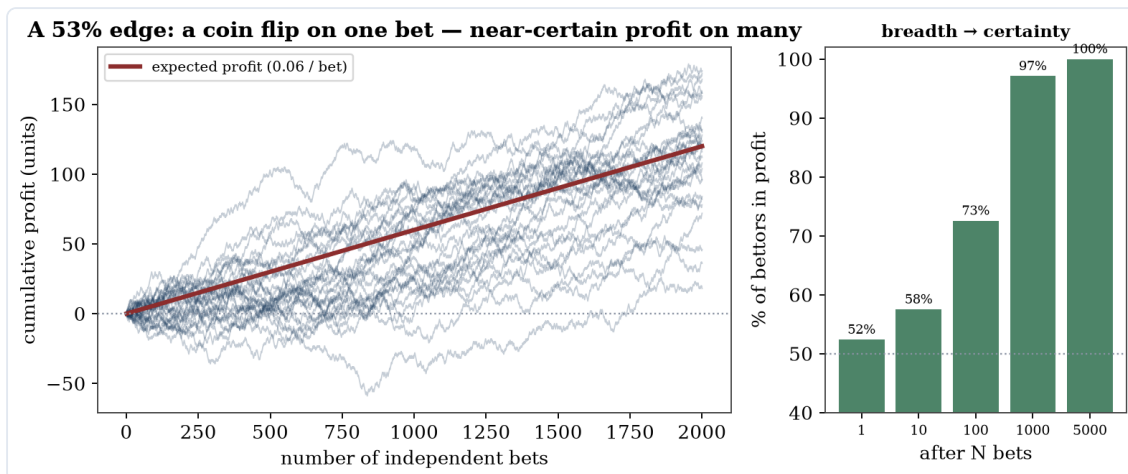
Figure 5 — The casino made concrete. Left: many gamblers with the same tiny 53% edge — on a few bets they scatter and some lose, but across thousands of independent bets they fan into reliable profit. Right: the share of them in profit climbs from a coin-flip toward certainty as the number of bets grows. A small edge and large breadth is the whole game.
