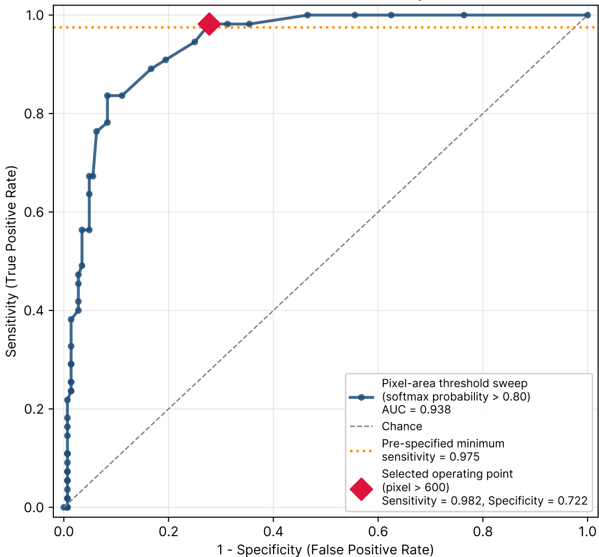
ROC Curve: Case-Level Abandoned Lead Detection (Out-of-Fold Predictions, Softmax Probability Threshold = 0.80)
